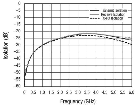
Figure 4. Typical Isolation
